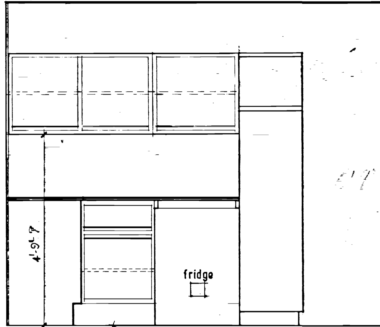
Section 2-2
