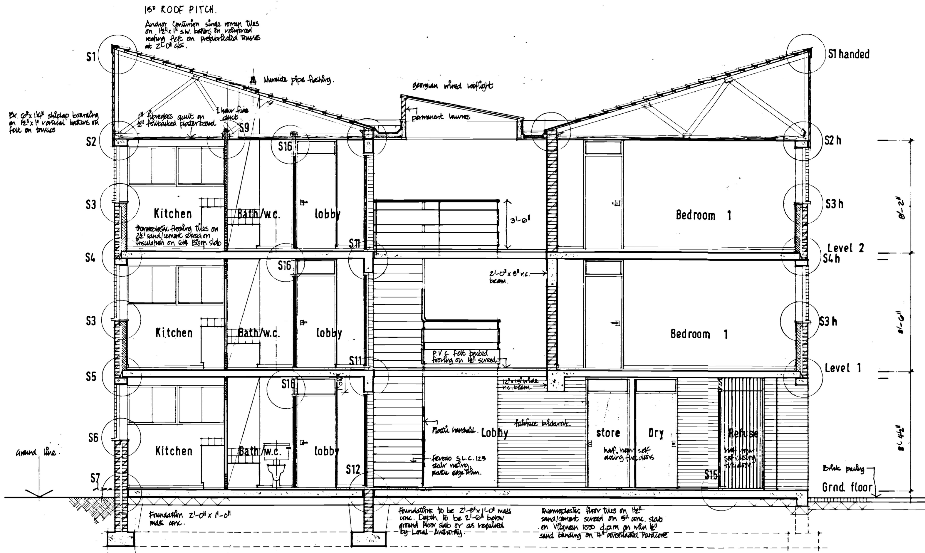
SECTION 1-1
