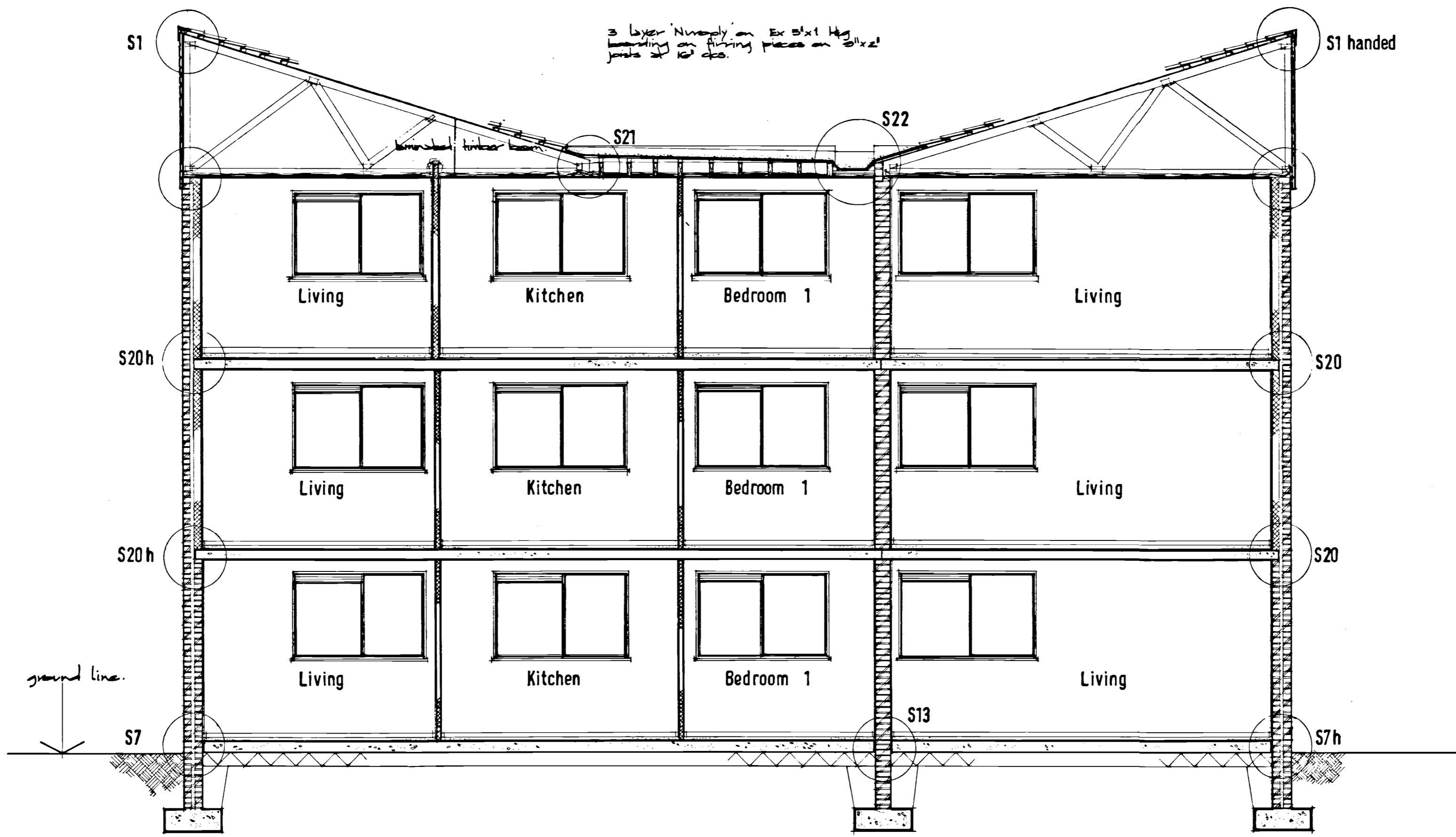
SECTION 5-5
