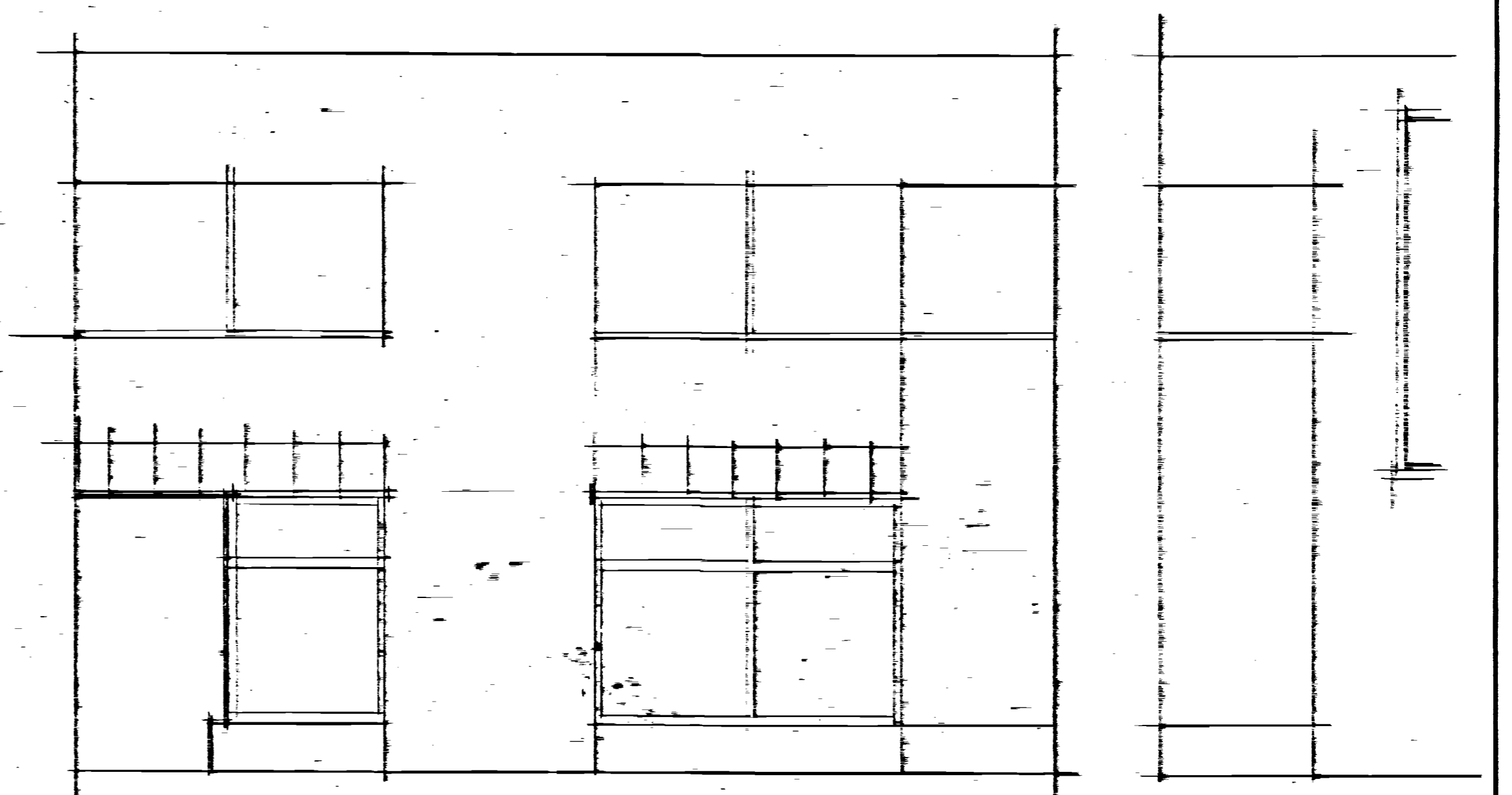
SECTION 3-3
