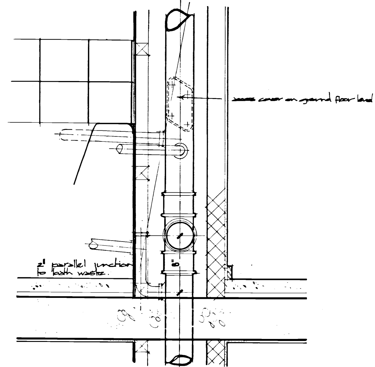
Detail 1
