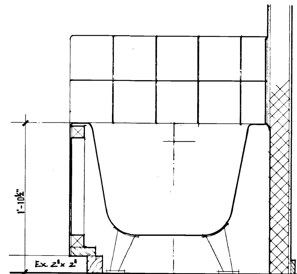
Detail 2
